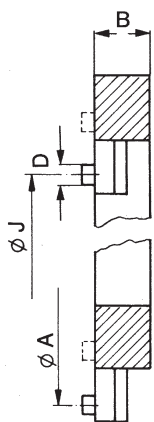
A09 Jaw cutting attachment for 3-jaw chucks
